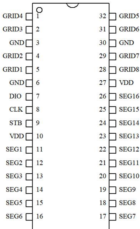
HTM1629A-TD 32SOP
