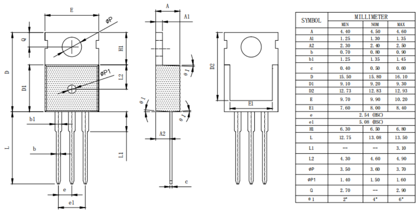
Figure 4. TO-220-FB
