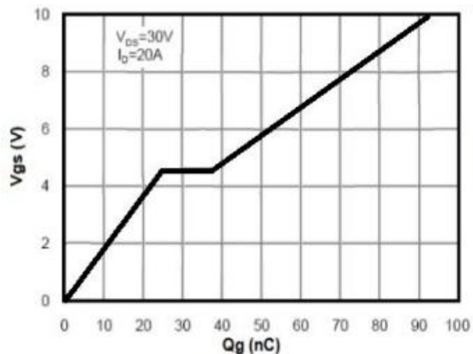
Figure 5 Gate Charge
