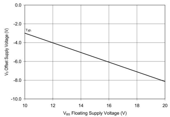
Figure 32. Maximum V_{\text{S}} Negative Offset vs V_{\text{BS}} Supply Voltage
