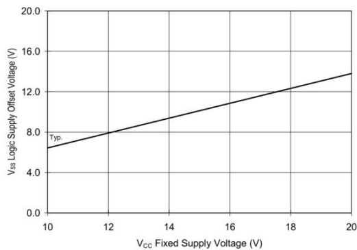
Figure 33. Maximum V_{\text{SS}} Positive Offset vs V_{\text{CC}} Supply Voltage
