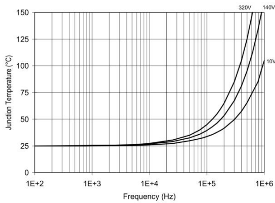
Figure 31. DOT7392N TJ vs. Frequency (IRFPE50) R_{\text{GATE}} = 10\Omega , V_{\text{CC}} = 15\text{V}
