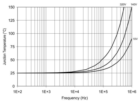
Figure 30. DOT7392N TJ vs. Frequency (IRFBC40) R_{\text{GATE}} = 15\Omega , V_{\text{CC}} = 15\text{V}
