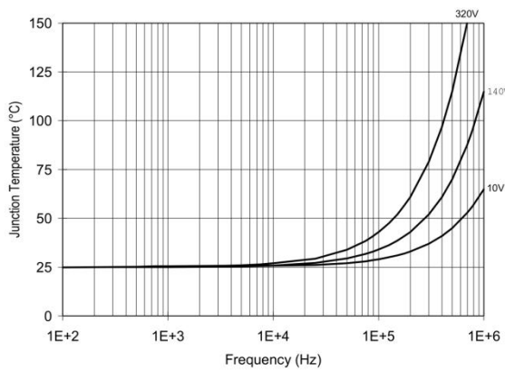
Figure 29. DOT7392N TJ vs. Frequency (IRFBC30) R_{\text{GATE}} = 22\Omega , V_{\text{CC}} = 15\text{V}
