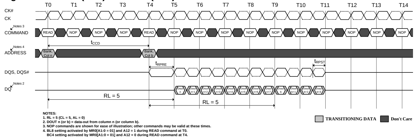
Figure 37. READ (BL8) to READ (BL4) OTF
