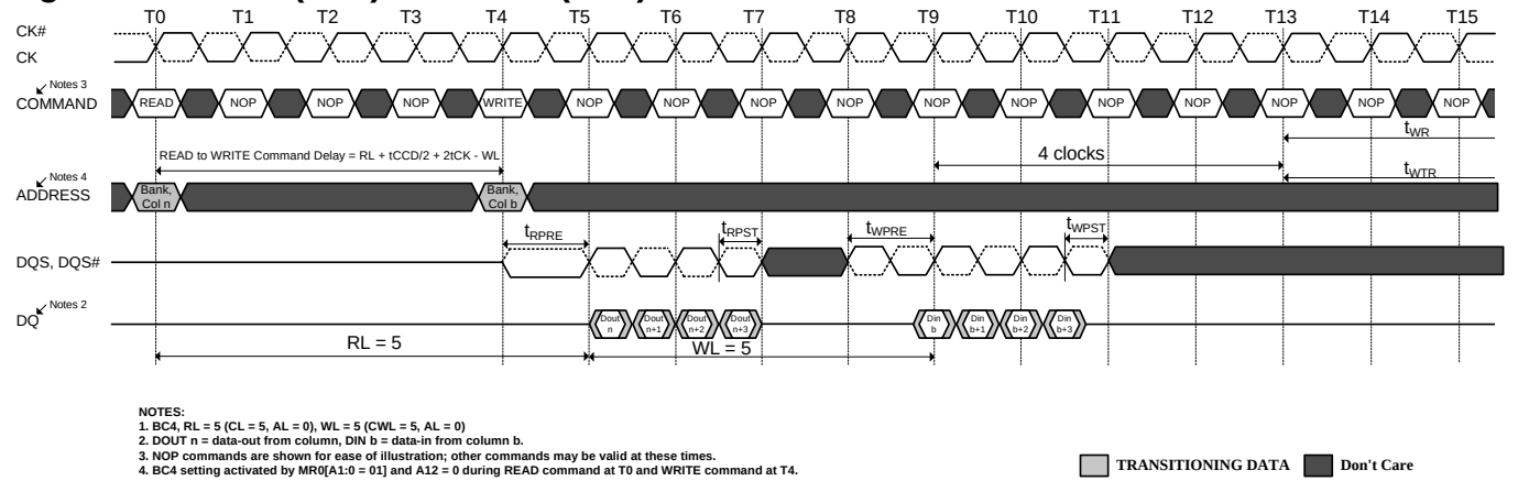
Figure 36. READ (BL4) to WRITE (BL4) OTF
