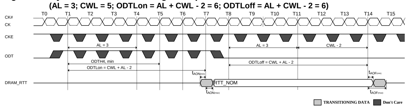
Figure 68. Synchronous ODT Timing Example
