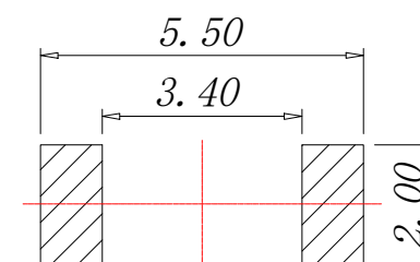
PCB.WELDING DRAWING
