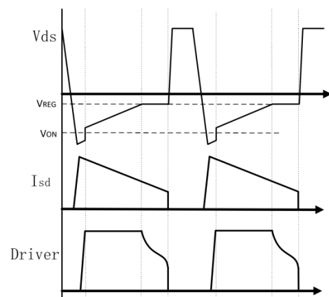
Figure 2 Operation in CCM mod
