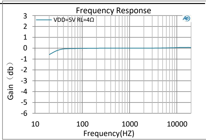
图6：Frequency Response
