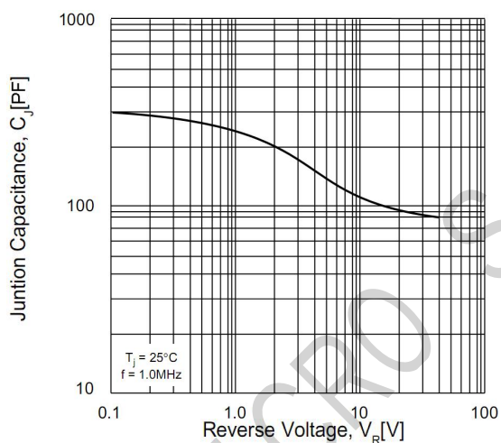
Figure 3. Junction Capacitance
