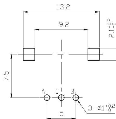
P.C.B.MOUNTING DETAIL
