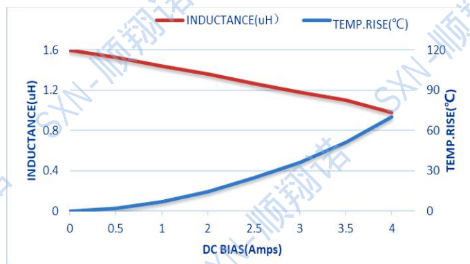
SMTC201610-1R5M
