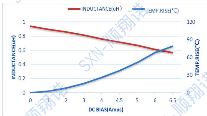
SMTC201610-1R0M
