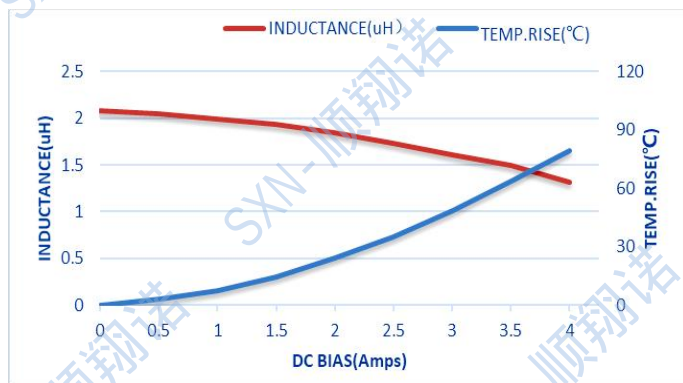
SMTC201610-2R2M
