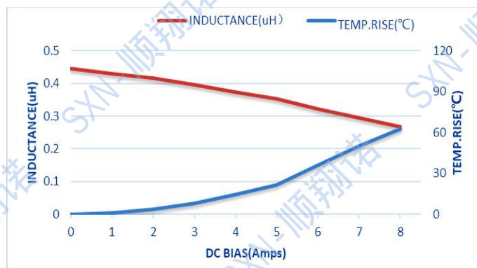
SMTC201610-R47M
