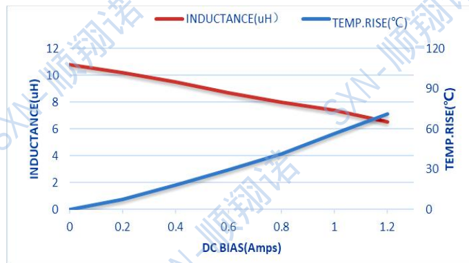
SMTC201610-100M
