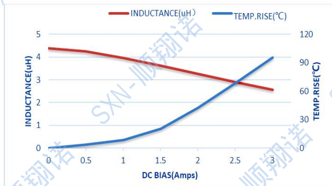
SMTC201610-4R7M
