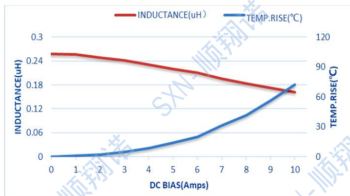
SMTC201610-R22M
