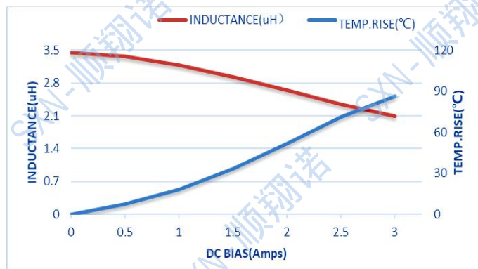
SMTC201610-3R3M
