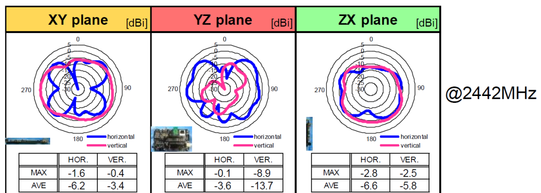
Figure 12 – Directivity for 1YN M.2 Module Mounted on iMX OEM Carrier Board
