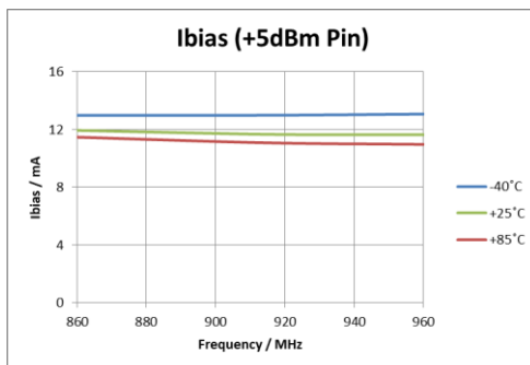
Figure 20: Ibias (+5 dBm Pin)
