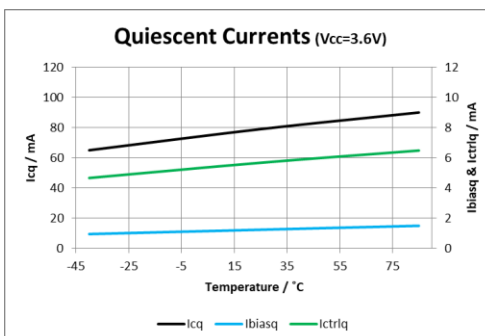
Figure 24: Quiescent Currents
