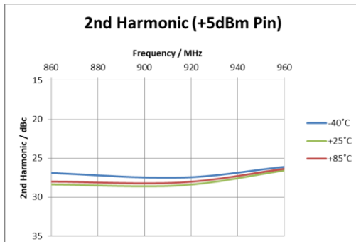
Figure 8: 2 nd Harmonic (+5 dBm Pin)
