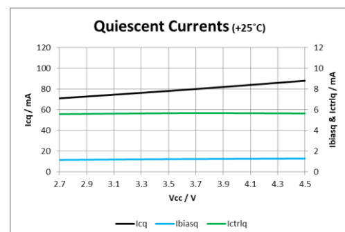
Figure 25: Quiescent Currents
