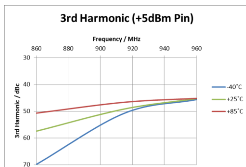
Figure 10: 3 rd Harmonic (+5 dBm Pin)
