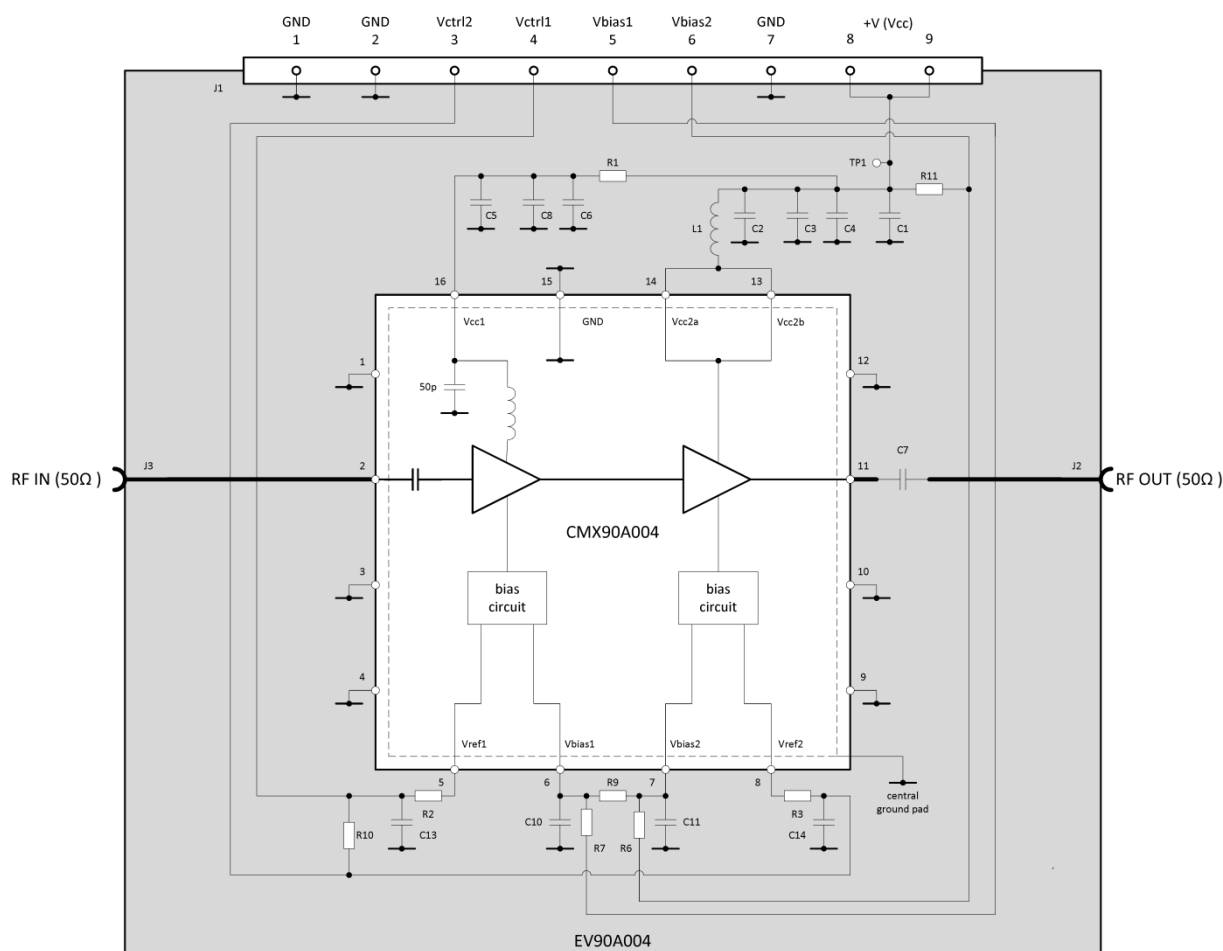
Figure 30: EV90A004 Schematic
