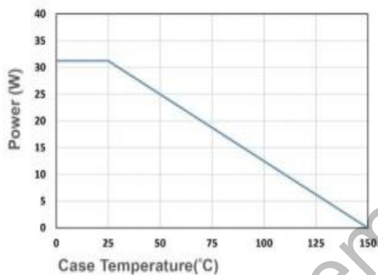
Figure 3. Power Dissipation
