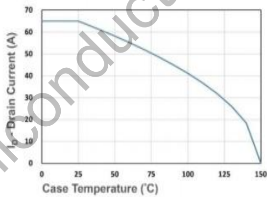
Figure 4. Drain Current
