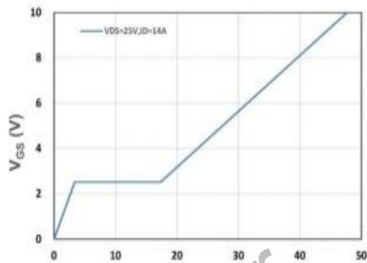
Figure 2. Gate Charge Characteristics
