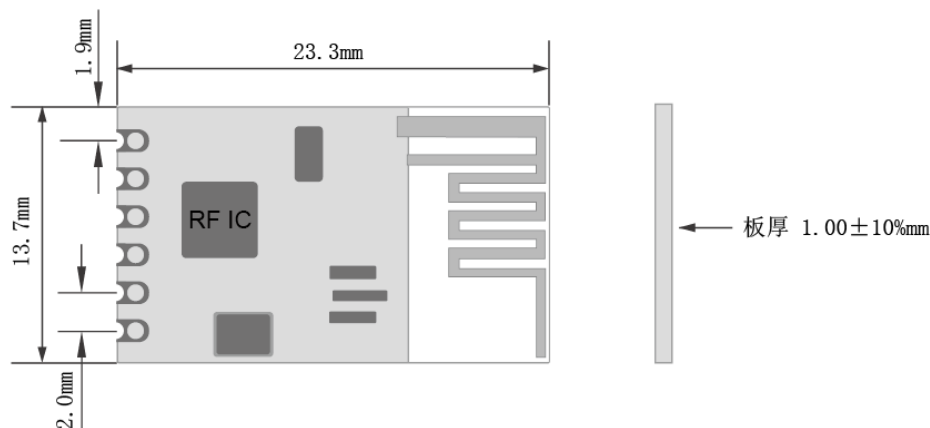
M-BK2461U Dimension
