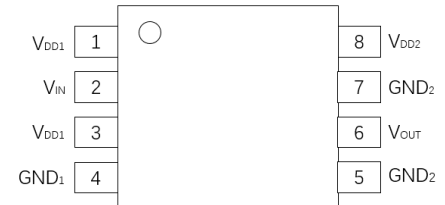
Figure 3. \pi 110M3x Pin Configuration
