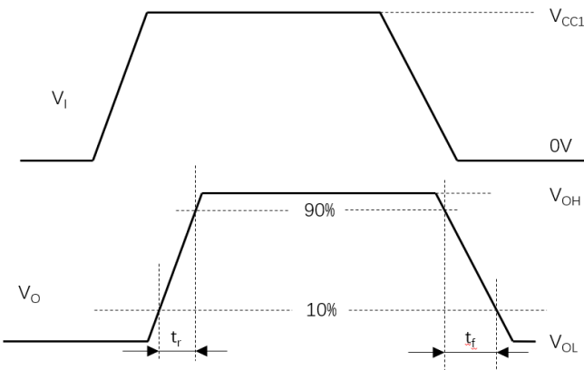
Figure 7. Transition time waveform measurement
