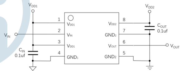
Figure 2. \pi 110M3x Typical Application Circuit
