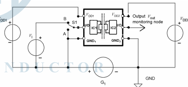
Figure 11. Common-mode transient immunity (CMTI) measurement
