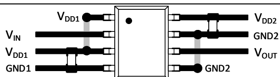
Figure 9. Recommended Printed Circuit Board Layout
