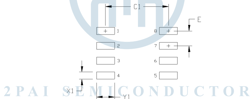
Figure 13.8-Lead Narrow Body SOIC [NB SOIC-8] Land Pattern
