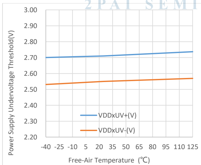
Figure 5. UVLO vs. Free-Air Temperature
