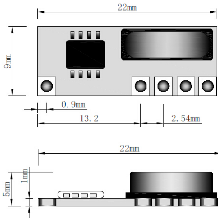
Figure 1: Module size
