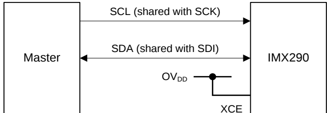
Pin connection of serial communication
