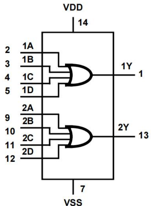
Figure 2.2 Functional Diagram
