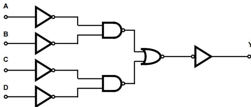
Figure 3.1: CD4072 Logic Diagram
