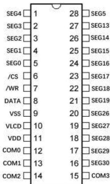
1621B 28SOP-A/SSOP-A
