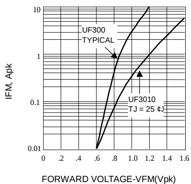
Fig. 2-FORWARD CHARACTERISTICS
