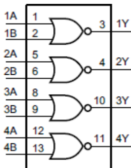
Figure 1. Functional diagram
