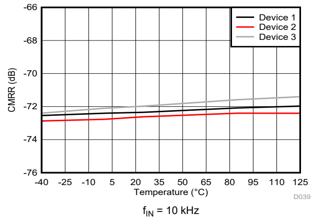
图 6-30. Common-Mode Rejection Ratio vs Temperature
