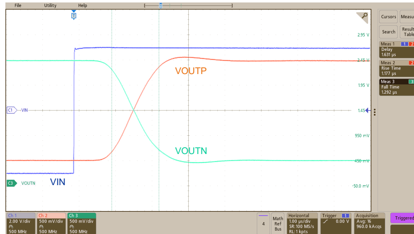
图 8-4. Step Response of the AMC1350
