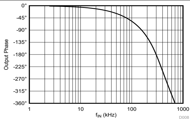
图 6-36. Output Phase vs Input Frequency
