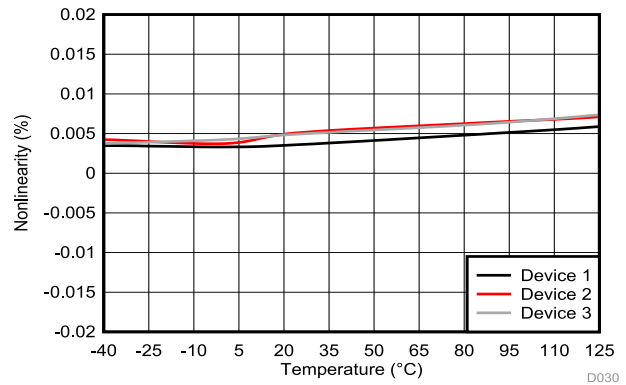
图 6-18. Nonlinearity vs Temperature
