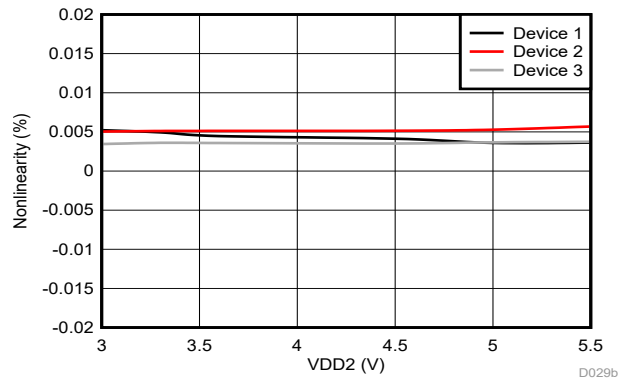
图 6-17. Nonlinearity vs Low-Side Supply Voltage
