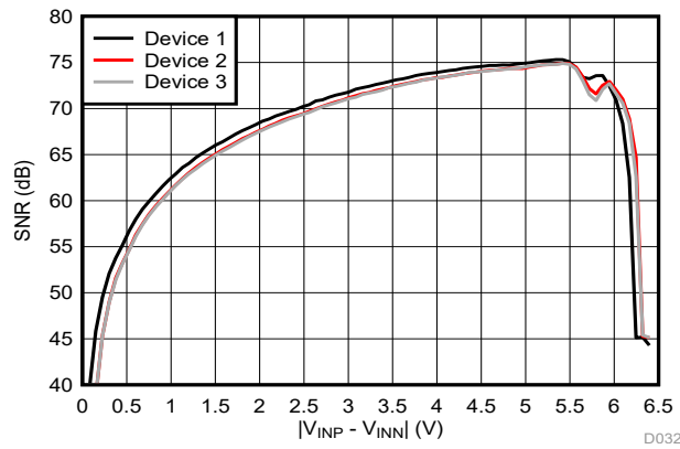
图 6-23. Signal-to-Noise Ratio vs Input Voltage
