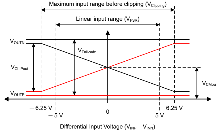
图 7-2. Output Behavior of the AMC1350
