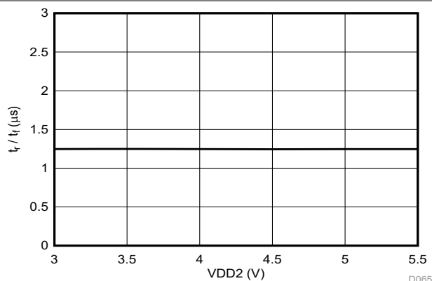
图 6-41. Output Rise and Fall Time vs Supply Voltage
