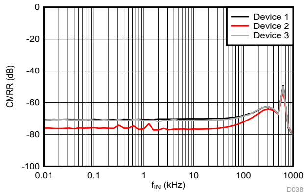
图 6-29. Common-Mode Rejection Ratio vs Input Frequency
