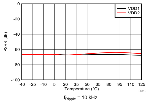
图 6-32. Power-Supply Rejection Ratio vs Temperature
