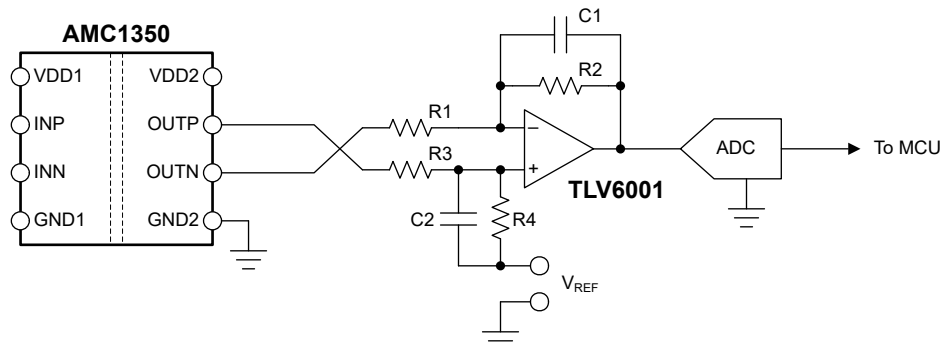
图 8-3. Connecting the AMC1350 Output to a Single-Ended Input ADC
