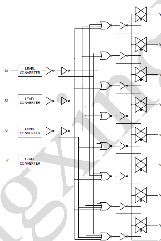
Figure 5. Logic diagram
