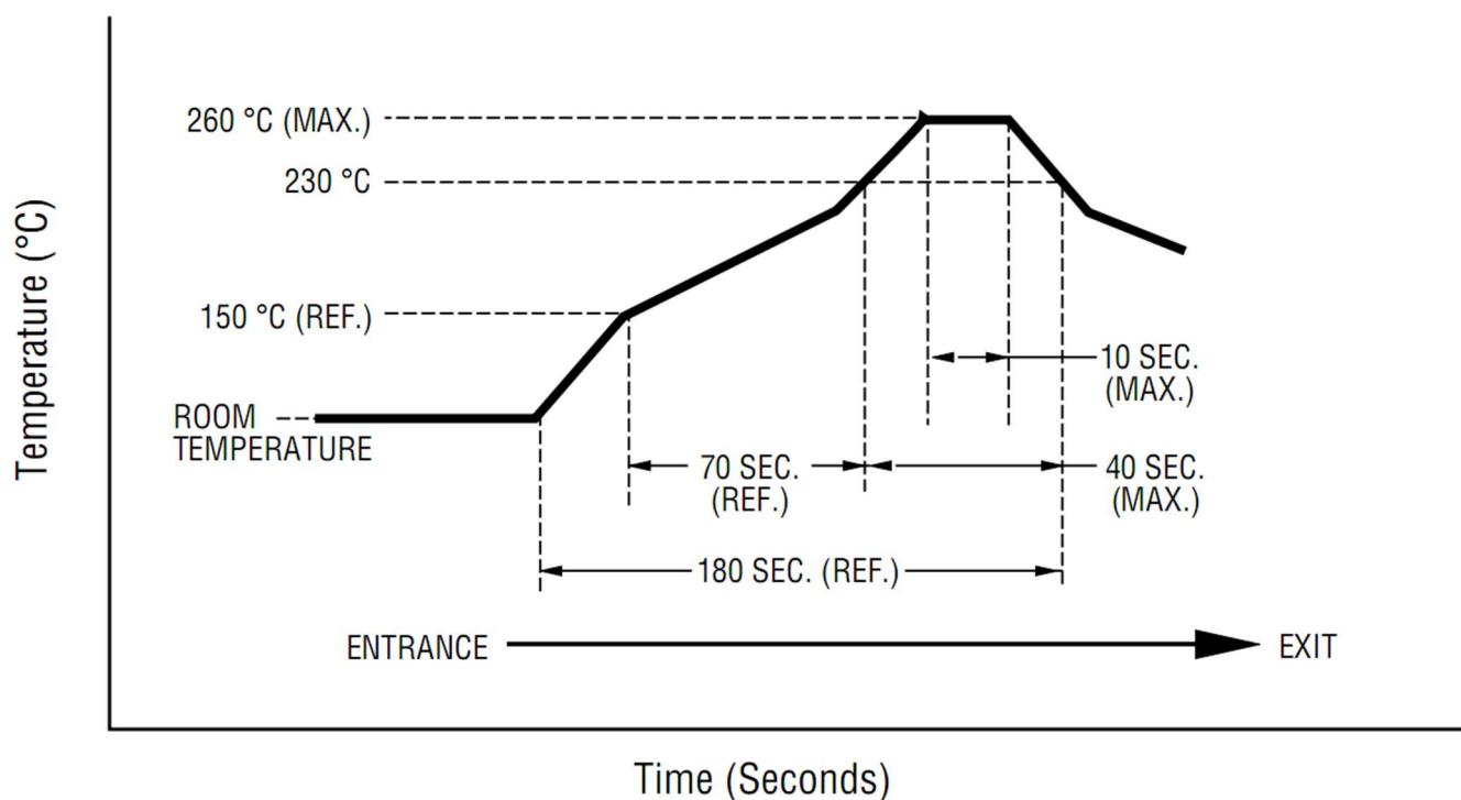
Figure 12. MHC0450L03 Thermal Reflow Profile
