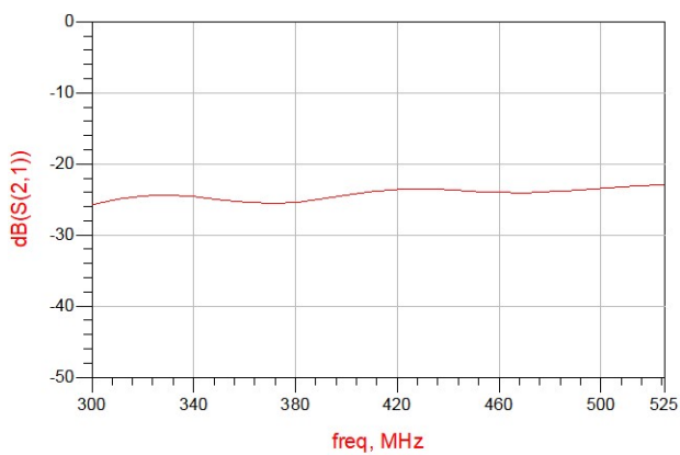
Figure 9. MHC0450L03 Isolation
