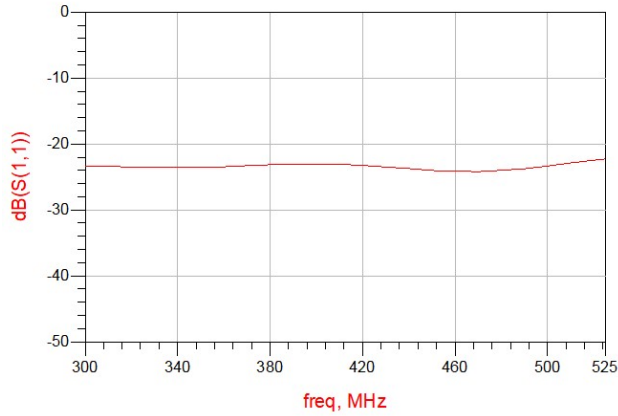
Figure 5. MHC0450L03 Return Loss (S11)
