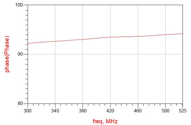
Figure 10. MHC0450L03 Phase
