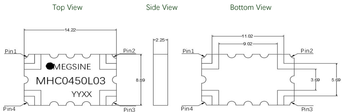
Figure 2. MHC0450L03 Outline Drawing
