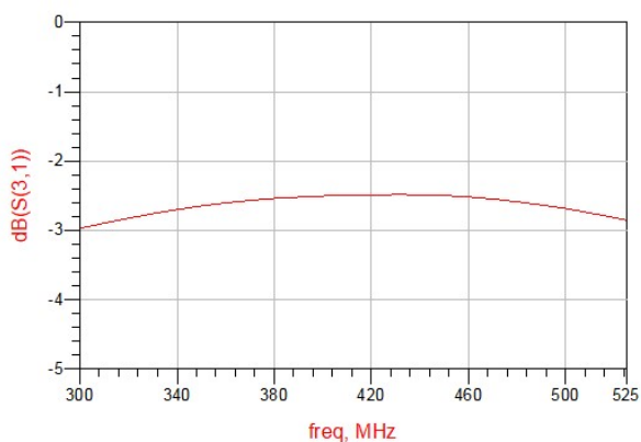
Figure 3. MHC0450L03 Coupling
