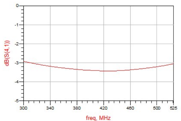
Figure 4. MHC0450L03 Transmission
