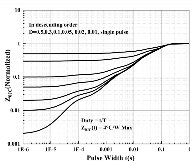
Figure 12. Normalized Transient Impedance
