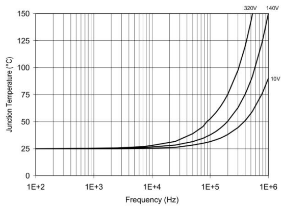
Figure 30. XL2110/XL2113 TJ vs. Frequency (IRFBC40) R_{GATE} = 15\Omega , V_{CC} = 15V
