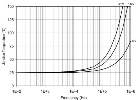
Figure 33. XL2110S/XL2113S TJ vs. Frequency (IRFBC30) R_{GATE} = 22\Omega , V_{CC} = 15V
