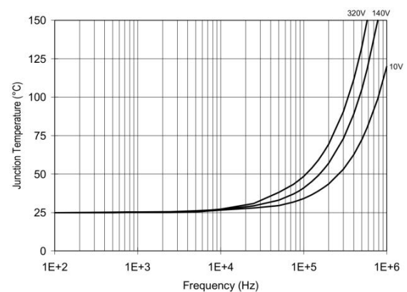
Figure 34. XL2110S/XL2113S TJ vs. Frequency (IRFBC40) R_{GATE} = 15\Omega , V_{CC} = 15V
