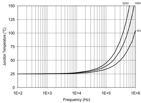
Figure 31. XL2110/XL2113 TJ vs. Frequency (IRFPE50) R_{GATE} = 10\Omega , V_{CC} = 15V
