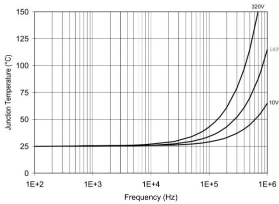
Figure 29. XL2110/XL2113 TJ vs. Frequency (IRFBC30) R_{GATE} = 22\Omega , V_{CC} = 15V
