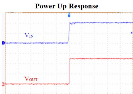
CH1: V_{IN} (5V/DIV) CH2: V_{OUT} (2V/DIV) I_{OUT}=10mA , V_{IN}=0V-10V 上电
