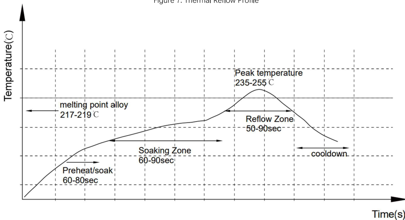
Figure 7. Thermal Reflow Profile
