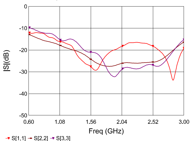
Figure 4. MPD0630W2 Return Loss
