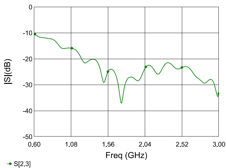
Figure 5. MPD0630W2 Isolation
