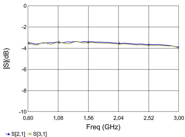
Figure 3. MPD0630W2 Insertion Loss
