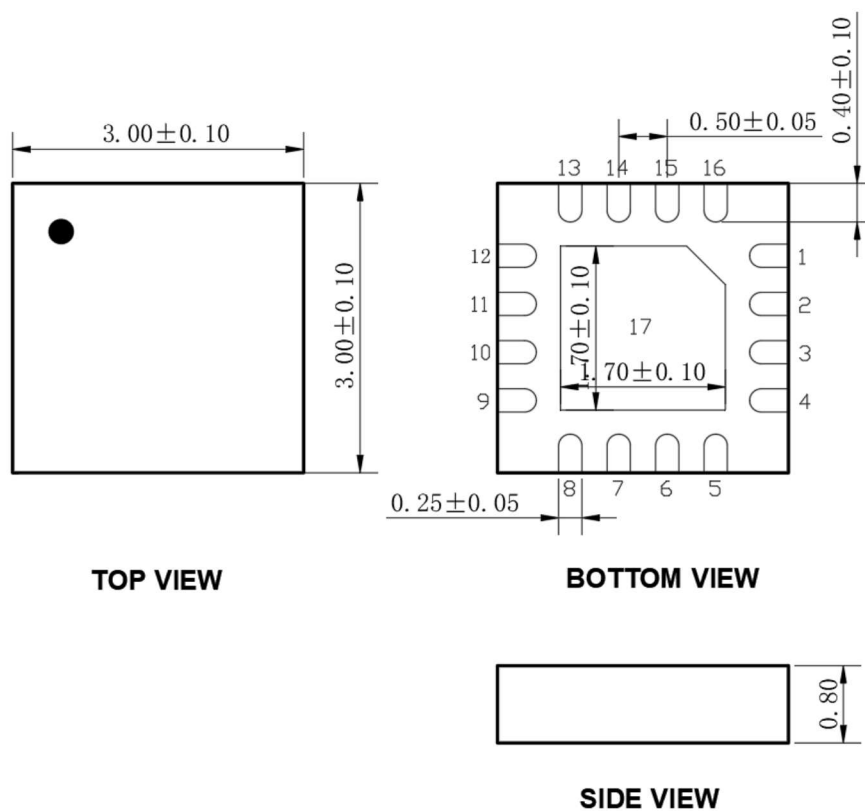
Figure 6. MPD0630W2 Outline Drawing
