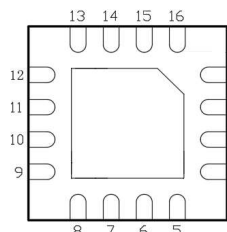
Figure 1.MPD0630W2 (Top View)
