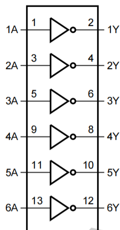
Figure 1. Functional diagram
