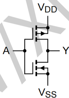
Figure 2. Schematic diagram (one inverter)
