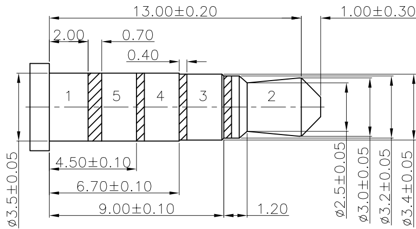
REF. Ø3.5mm 5POLE PLUG
