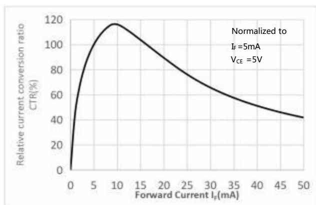
Fig.1 Relative Current Transfer Ratio vs. Forward Current
