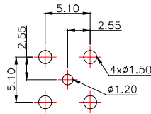
PCB WELDING DRAWING (TOLERANCE:±0.05)
