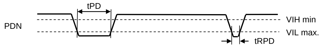
Figure 31. Power-down & Reset Timing
