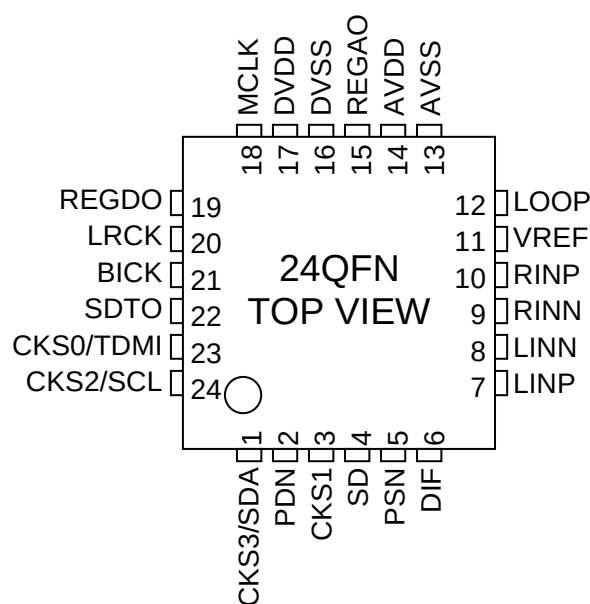
Figure 2. Pin Configurations
