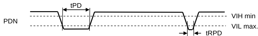
Figure 21. Power-down & Reset Timing
