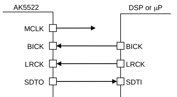
Figure 34. PLL Slave Mode
