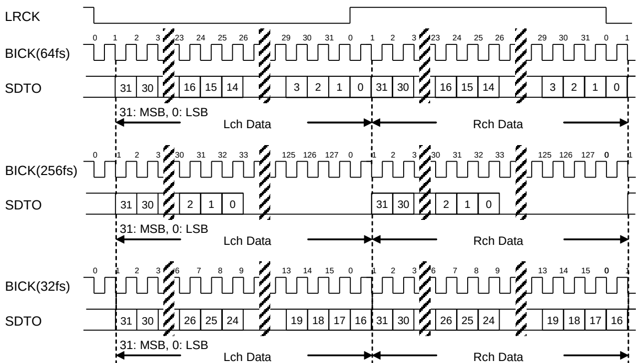
Figure 41. Stereo Output Timing (I²S Compatible)
