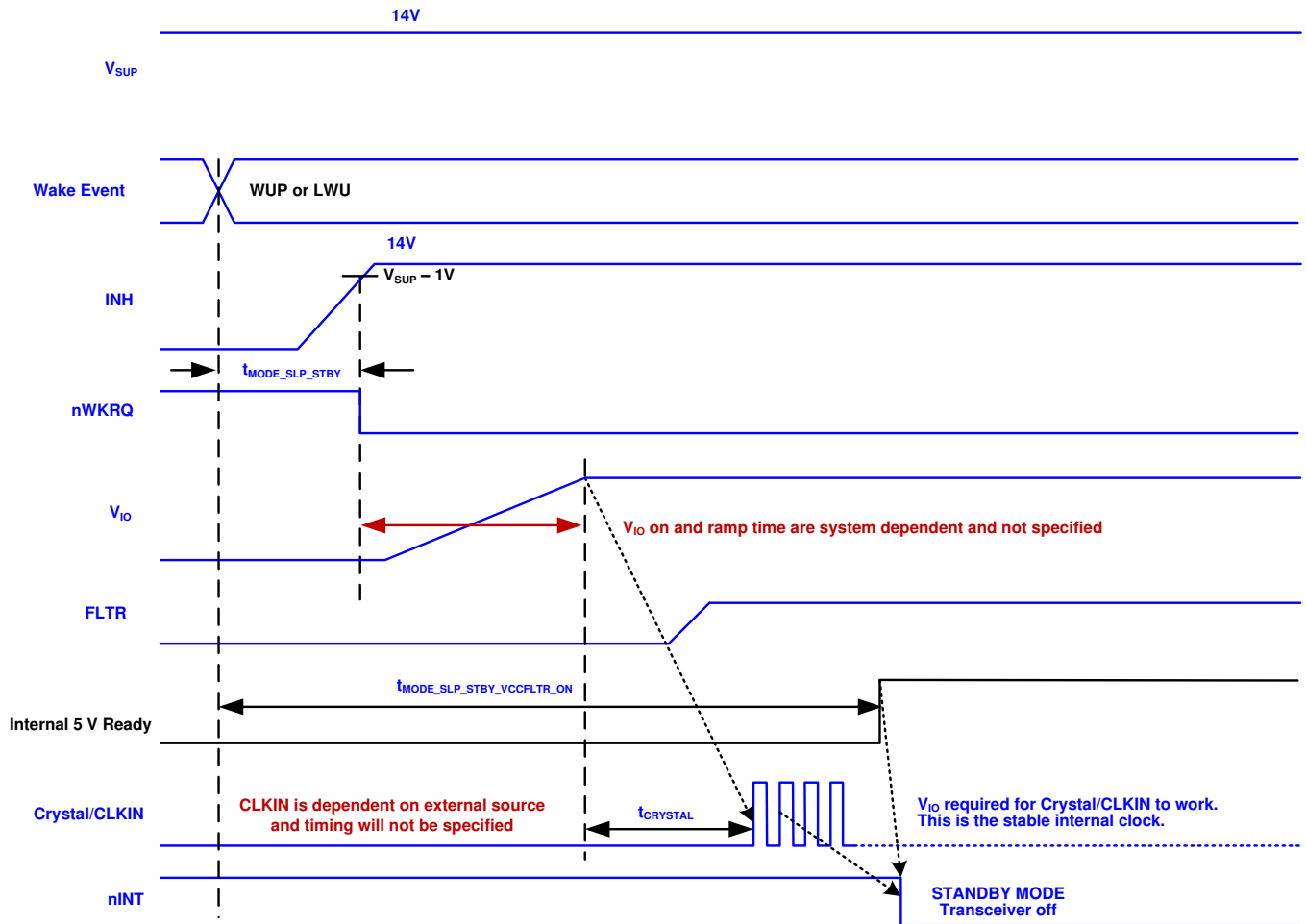
图 15. Sleep to Standby Timing
