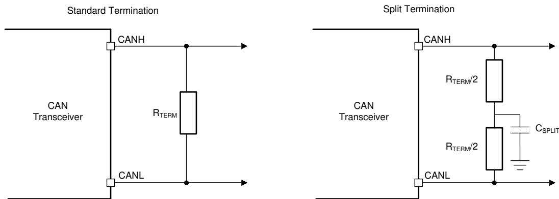
图 102. CAN Bus Termination Concepts
