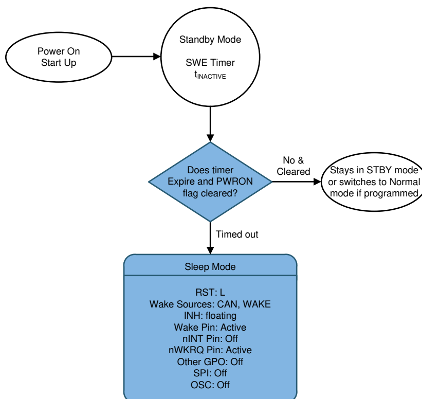
图 31. Power On Fail-safe Feature
