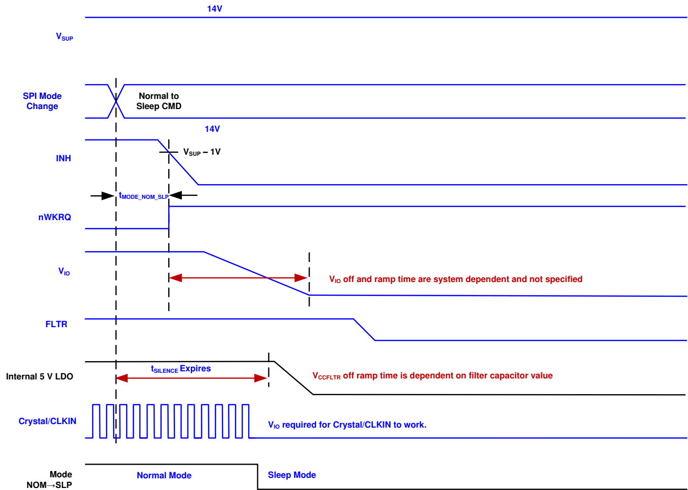
图 16. Normal to Sleep Timing
