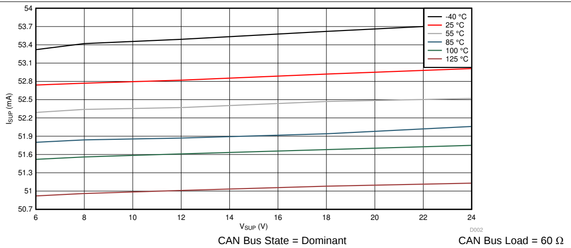
图 108. I_{SUP} Across V_{SUP} and Temperature
