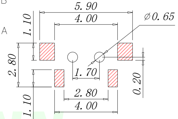
PCB.WELDING DRAWING
