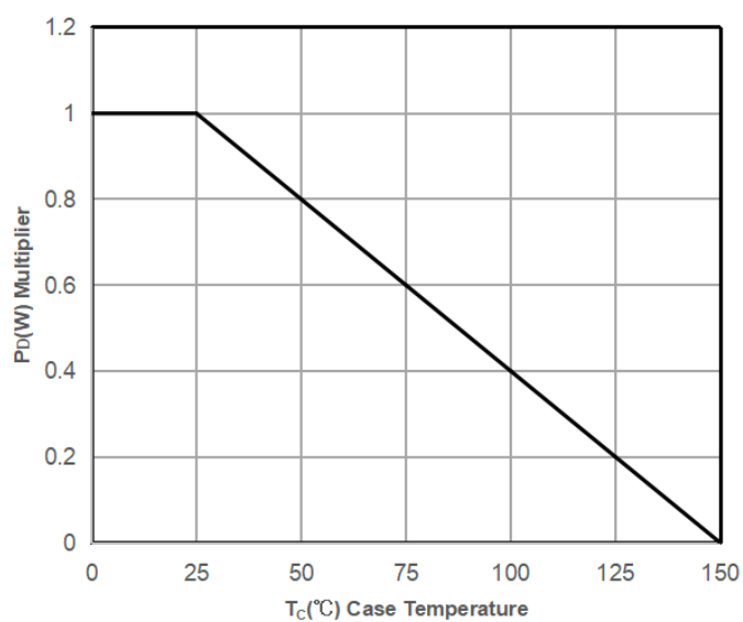
Power Dissipation P_{tot}=f(T_C)
