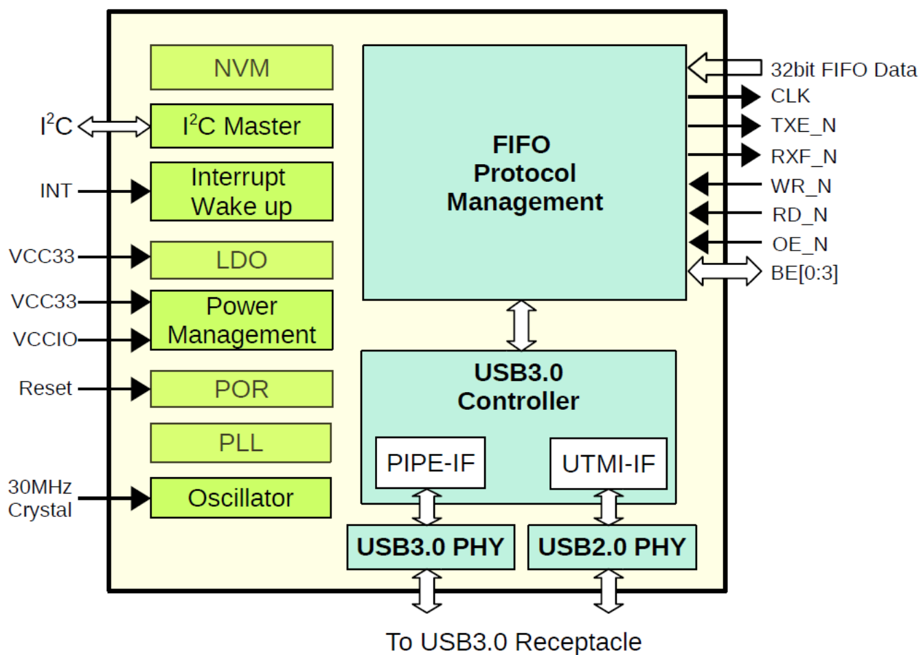
Figure 2.1 Block Diagram
