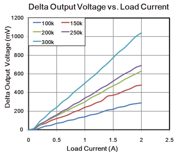
Figure 1. Delta Output Voltage vs. Load Current
