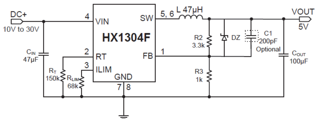
Application1: No Output Cable Resistance Compensation
