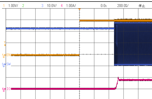
Figure 13.1.a V_{\text{IN}}=36\text{V} , I_{\text{OUT}}=800\text{mA} , 3pcs LED Series
