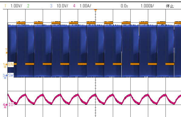
Figure 13.2.b LGS63042, V_{\text{IN}}=36\text{V} , I_{\text{OUT}}=800\text{mA} , 3pcs LED Series
