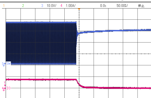
Figure 13.3.a V_{\text{IN}}=36\text{V} , I_{\text{OUT}}=800\text{mA} , 3pcs LED Series
