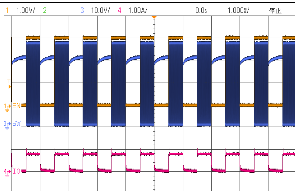
Figure 13.2.a LGS63040, V_{\text{IN}}=36\text{V} , I_{\text{OUT}}=800\text{mA} , 3pcs LED Series
