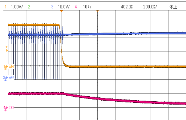
Figure 14.1.b V_{\text{IN}}=36\text{V} , I_{\text{OUT}}=10\text{mA} , 3pcs LED Series
