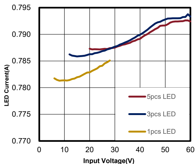
Figure 11.2.b I_{OUT}=800mA
