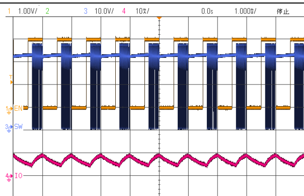
Figure 14.2.b LGS63042, V_{\text{IN}}=36\text{V} , I_{\text{OUT}}=10\text{mA} , 3pcs LED Series
