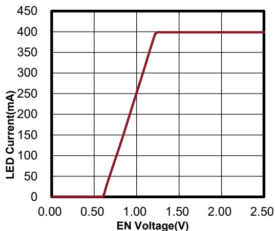
Figure 12.1.a LGS63040, V_{IN}=30V , 3pcs LED Series
