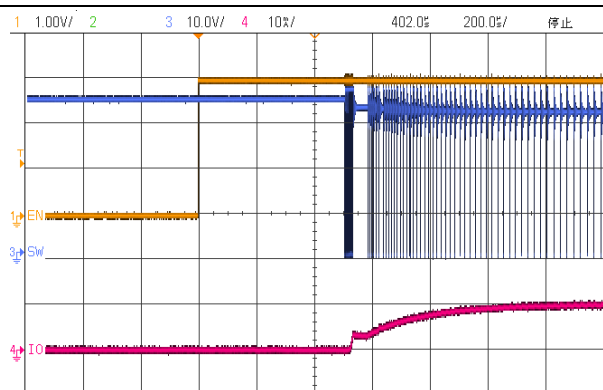
Figure 14.1.a V_{\text{IN}}=36\text{V} , I_{\text{OUT}}=10\text{mA} , 3pcs LED Series
