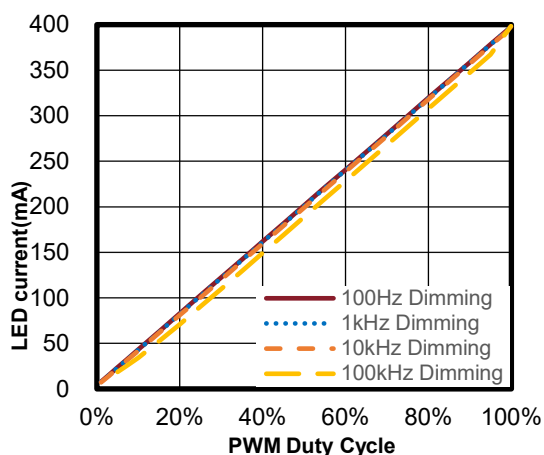
Figure 12.2.a LGS63042, V_{IN}=30V , 3pcs LED Series
