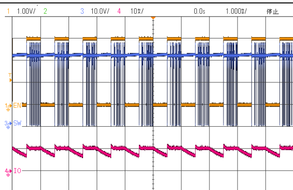
Figure 14.2.a LGS63040, V_{\text{IN}}=36\text{V} , I_{\text{OUT}}=10\text{mA} , 3pcs LED Series
