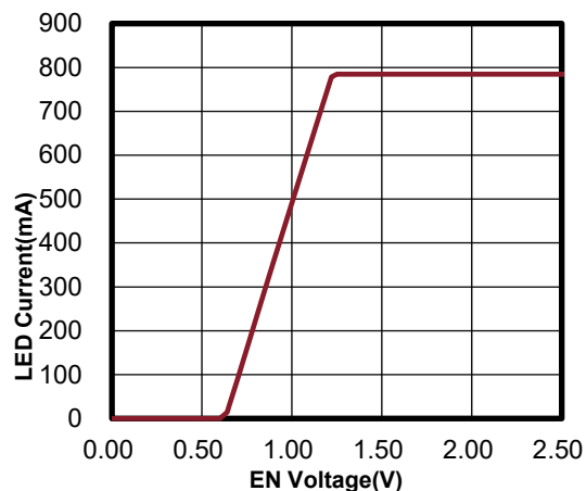
Figure 12.1.b LGS63040, V_{IN}=30V , 3pcs LED Series
