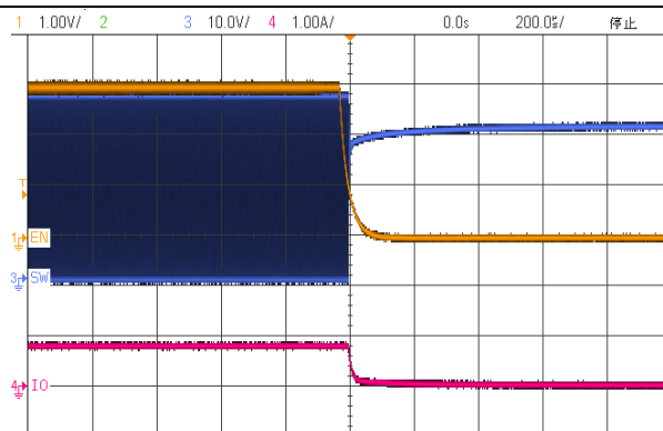
Figure 13.1.b V_{\text{IN}}=36\text{V} , I_{\text{OUT}}=800\text{mA} , 3pcs LED Series
