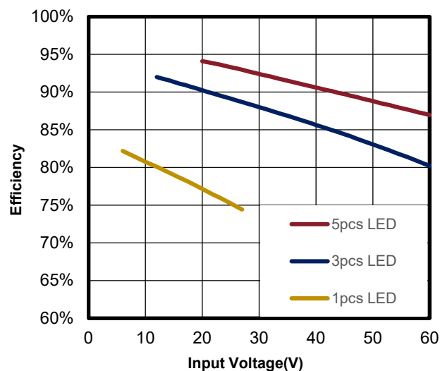
Figure 11.1.b I_{OUT}=800mA
