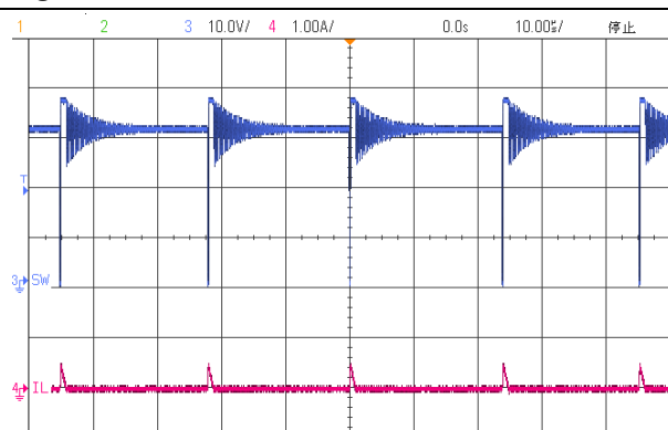
Figure 14.3.b V_{\text{IN}}=36\text{V} , I_{\text{OUT}}=10\text{mA} , 3pcs LED Series, Pulse Skip Mode
