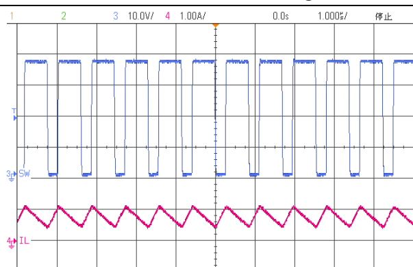
Figure 14.3.a V_{\text{IN}}=36\text{V} , I_{\text{OUT}}=800\text{mA} , 3pcs LED Series, CCM Mode
