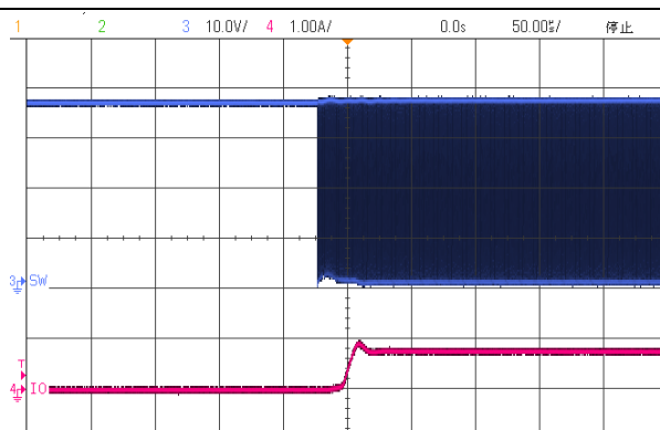
Figure 13.3.b V_{\text{IN}}=36\text{V} , I_{\text{OUT}}=800\text{mA} , 3pcs LED Series
