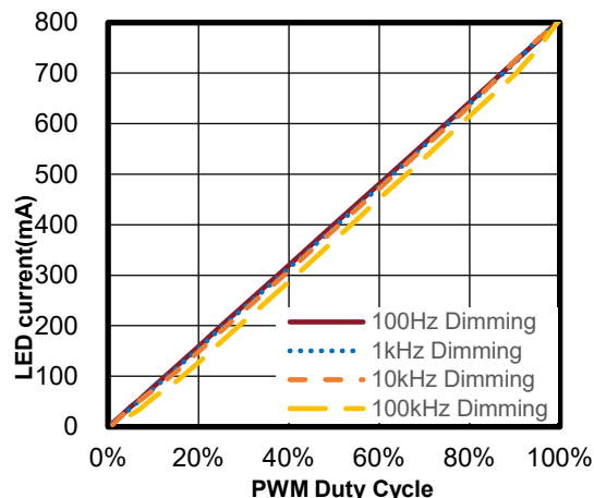
Figure 12.2.b LGS63042, V_{IN}=30V , 3pcs LED Series
