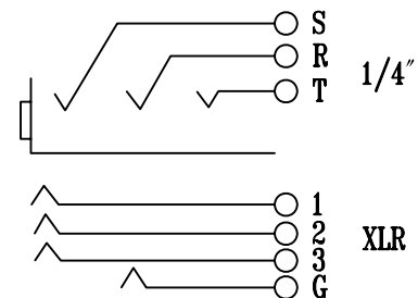
SCHEMATIC
