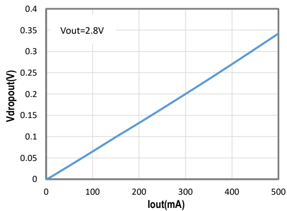
Vdropout Vs. Iout
