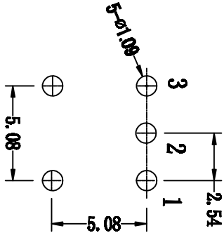
PC MOUNTING
