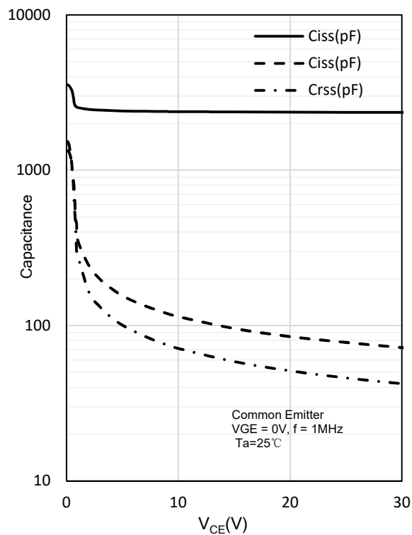
Fig. 8 Capacitance characteristics
