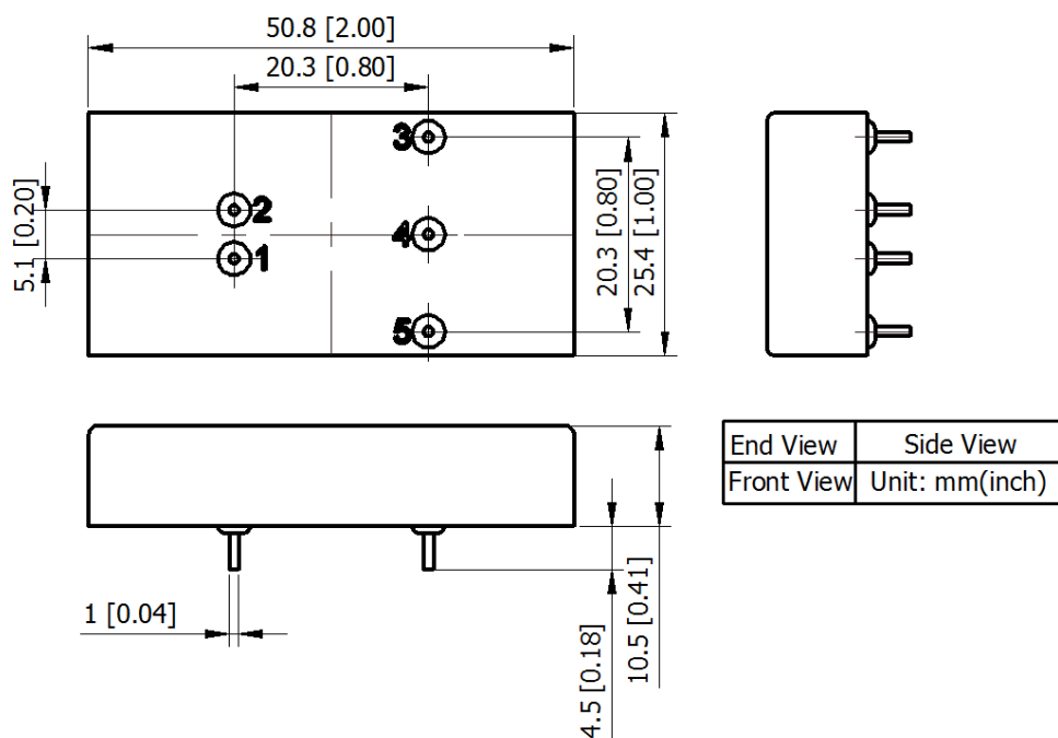
Figure 7. Outline Dimensions
