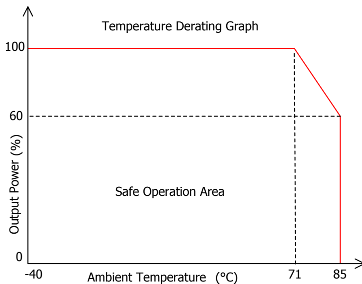
Figure 5. Derating Curve
