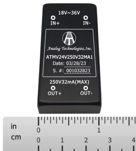
Figure 1. Top View
