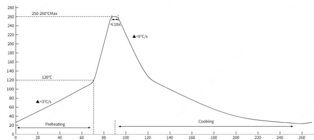
波峰焊 Wave-Soldering Profile
