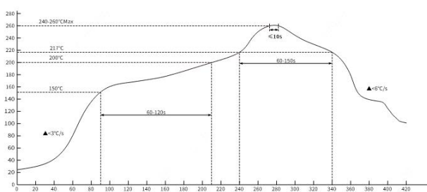
回流焊 IR Reflow-Soldering Profile
