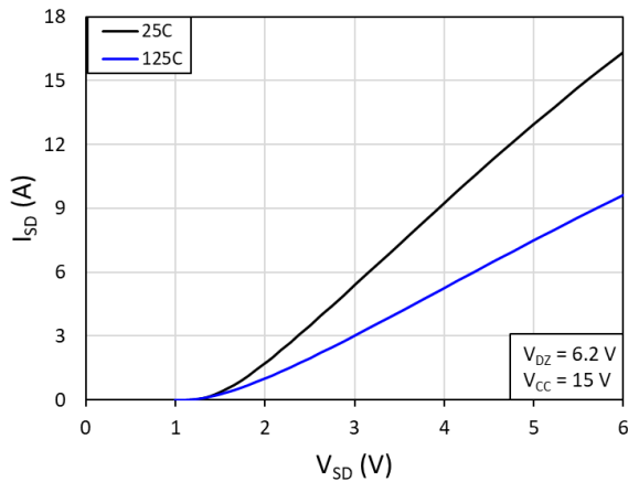
Fig. 5. Source-to-drain reverse conduction voltage vs. source-to-drain current at T = 25^\circ\text{C} and 125^\circ\text{C}
