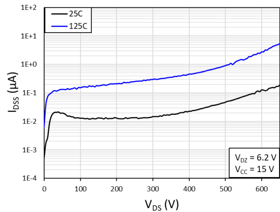
Fig. 6. Drain-to-source leakage current ( I_{DSS} ) vs. drain-to-source voltage ( V_{DS} ) at T = 25^\circ\text{C} and 125^\circ\text{C}
