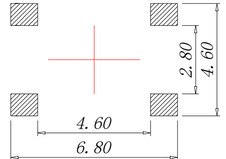
PCB.WELDING DRAWING
