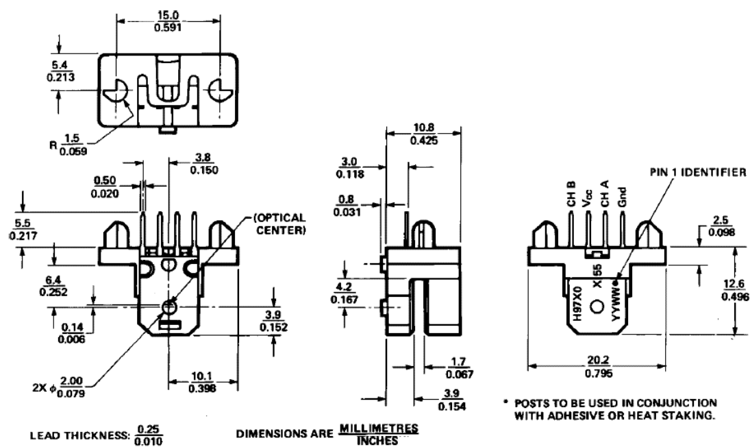
Mounting Option #55 – Backplane with Posts (Backplane Mounting)
