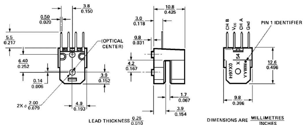
Mounting Option #54 – Tabless (Baseplane Mounting)
