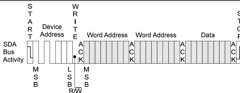
Figure 1-6. Byte Write
