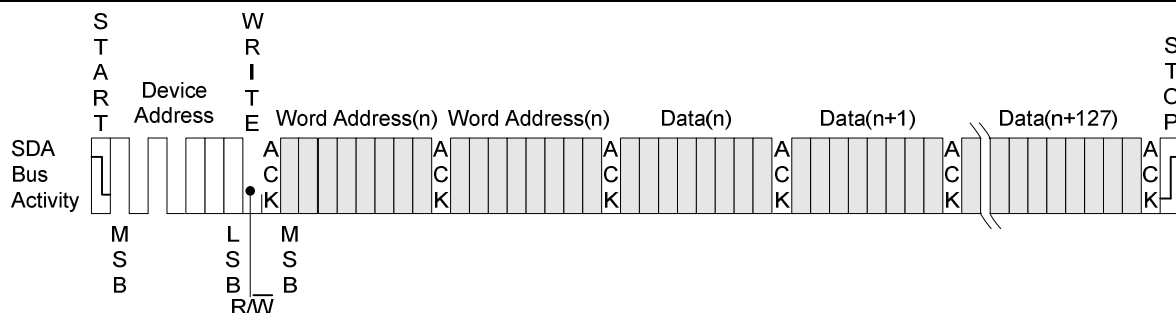
Figure 1-7. Page Write
