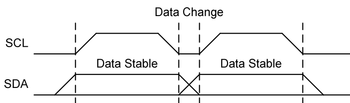
Figure 1-4. Data Validity Protocol
